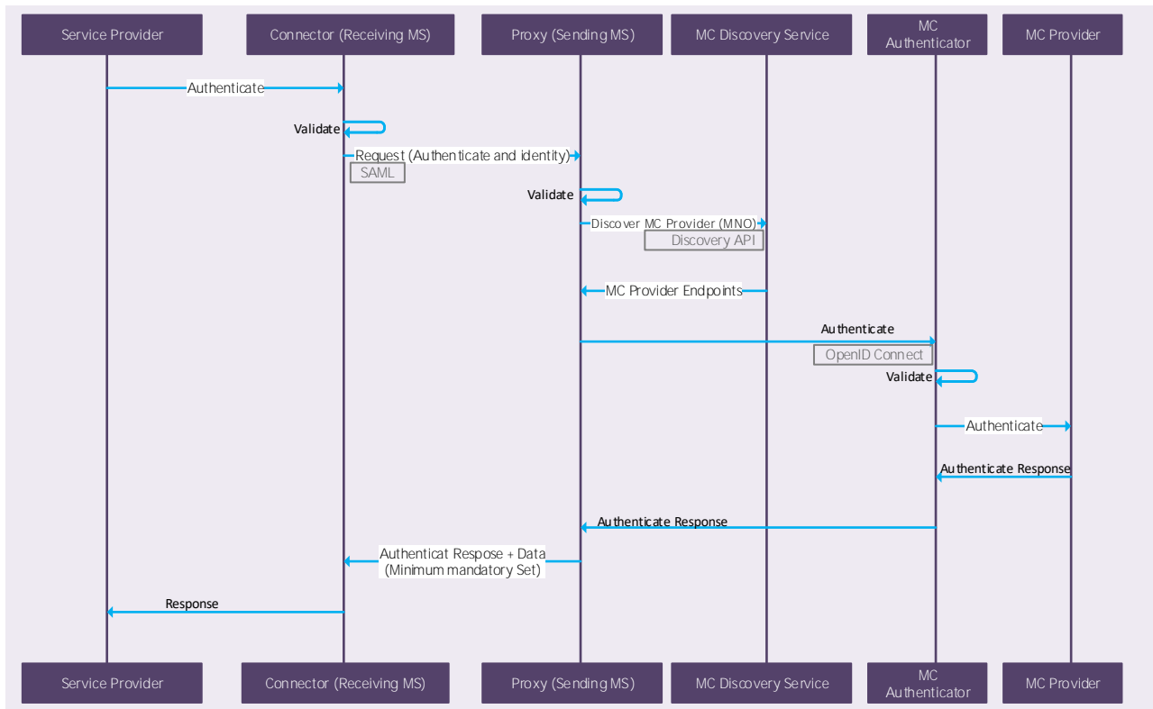
Figure 9 shows a flowchart of Mobile Connect used within an eIDAS deployment.
