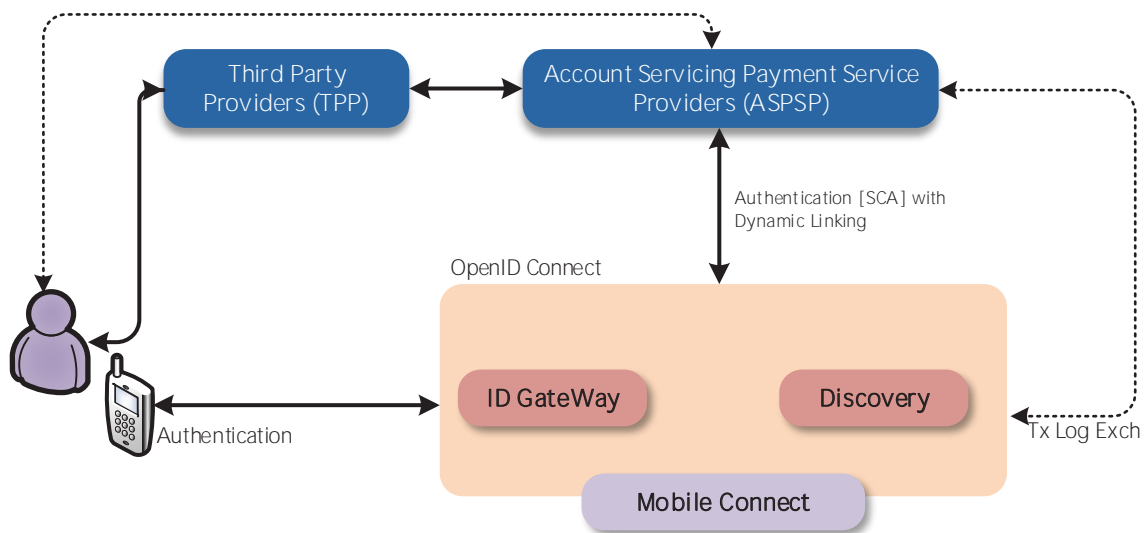
Figure 11 – High Level Reference Architecture for PSD2
