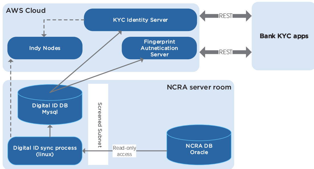
Figure 27 - NCRA Identity Infrastructure
