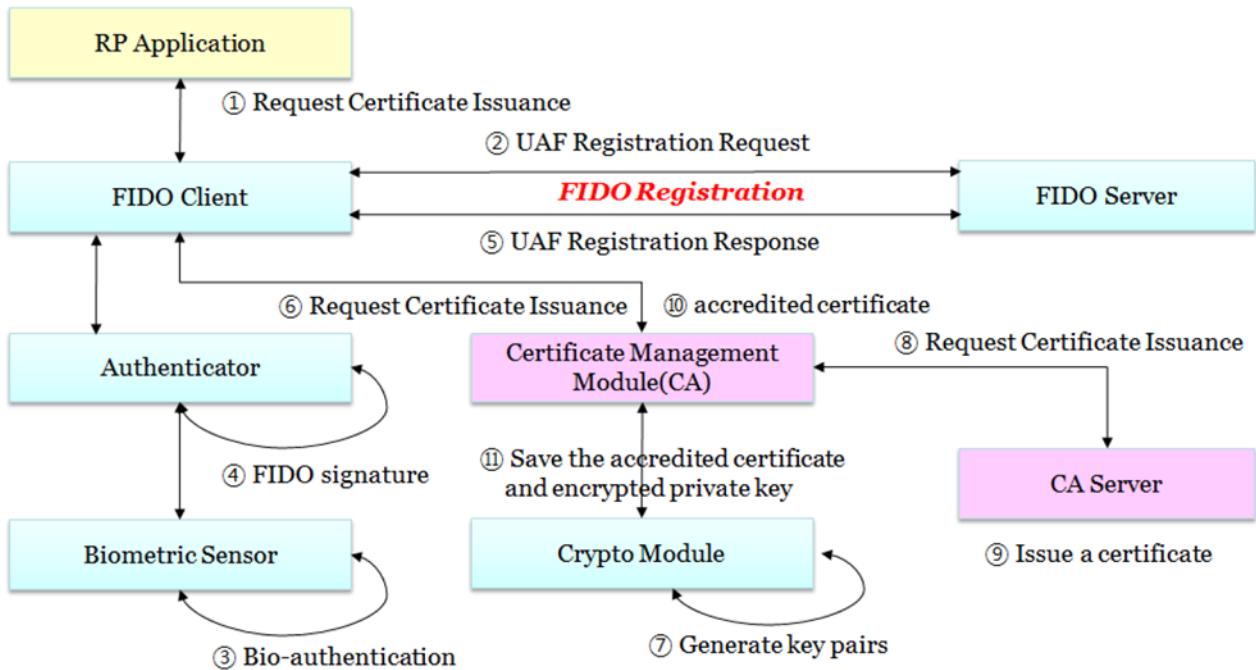
Figure 31 – Registration process of K-FIDO service
