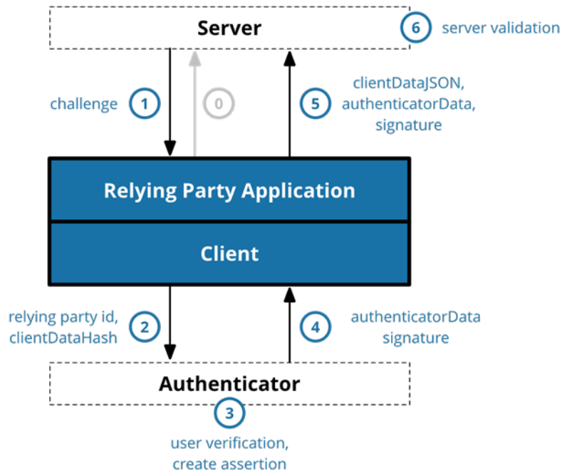
Figure 39 – Authentication process of FIDO
