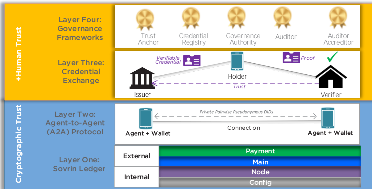
Figure 23 – Sovrin Infrastructure Layers
