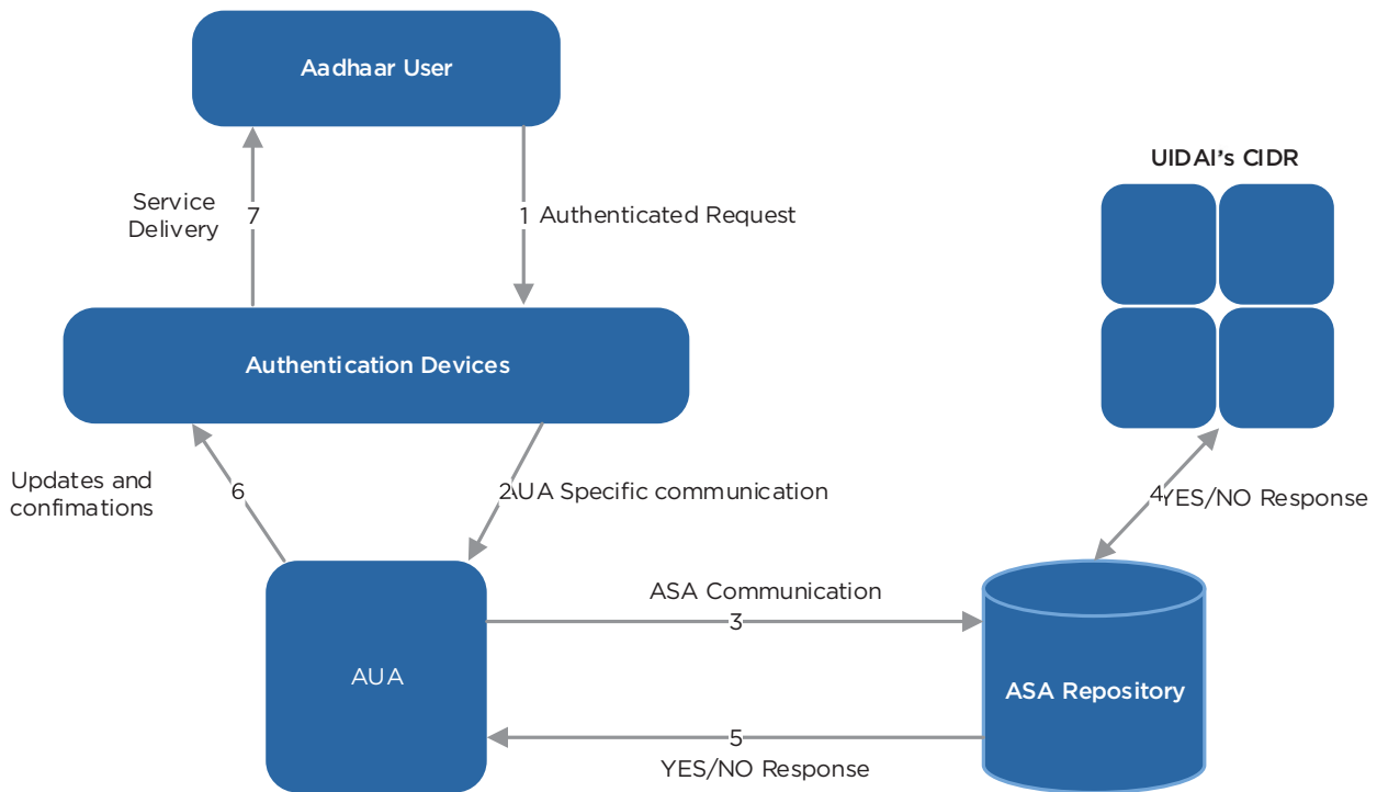
Figure 36 - Technical process of Authentication & e-KYC services
