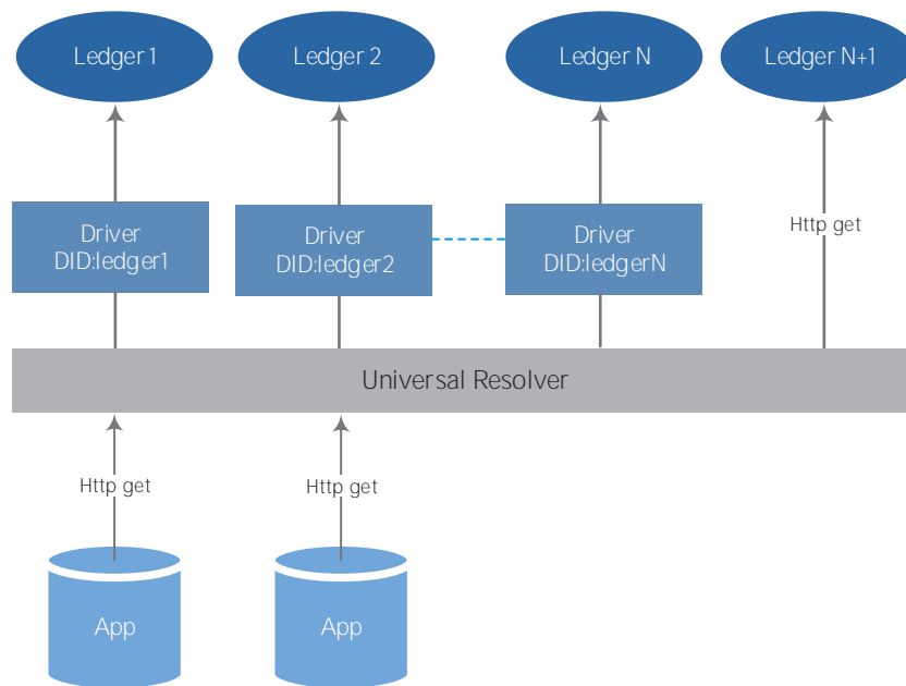
Figure 25 - Universal DID Resolver
