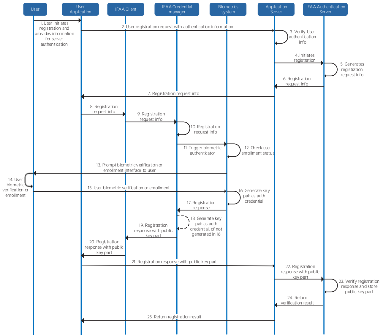
Figure 15 - IFAA biometric authentication - local model - Registration
