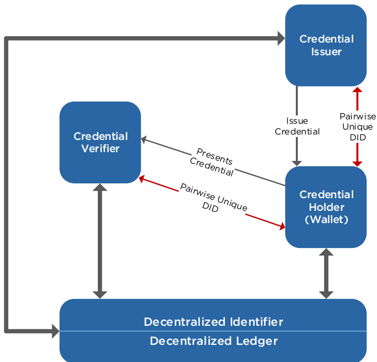
Figure 26 - Decentralized Identity Wallet with Verifiable Claims
