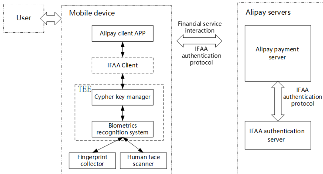
Figure 35 - IFAA use case: Alipay fingerprint/face payment - Technical framework
