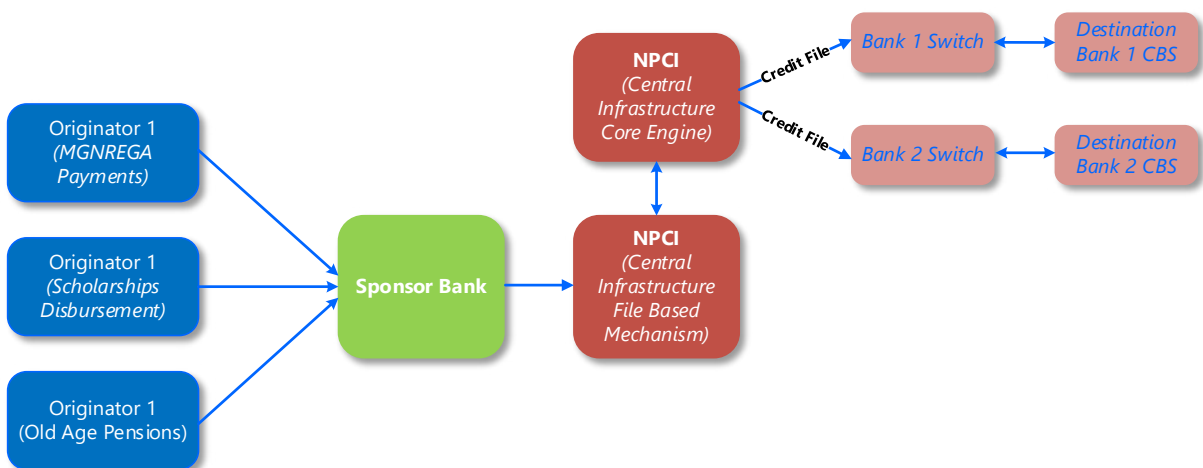
Figure 20 - Aadhaar Payments Bridge Process
