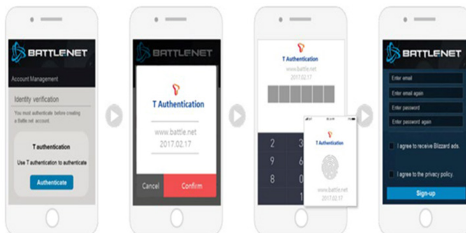
Figure 38 – User Journey to Authenticate to a Gaming Account Using T-Auth
