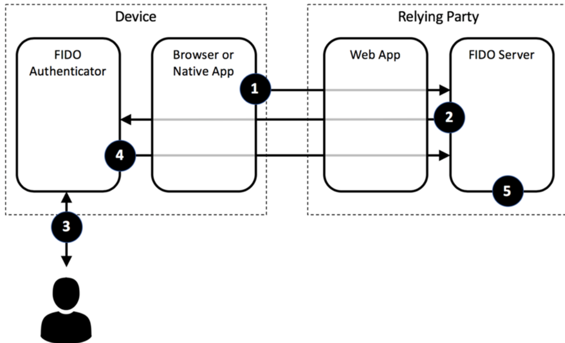
Figure 5 - FIDO Authentication
