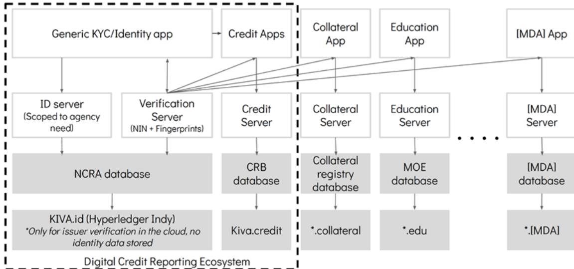
Figure 29 - Ecosystem Architecture
