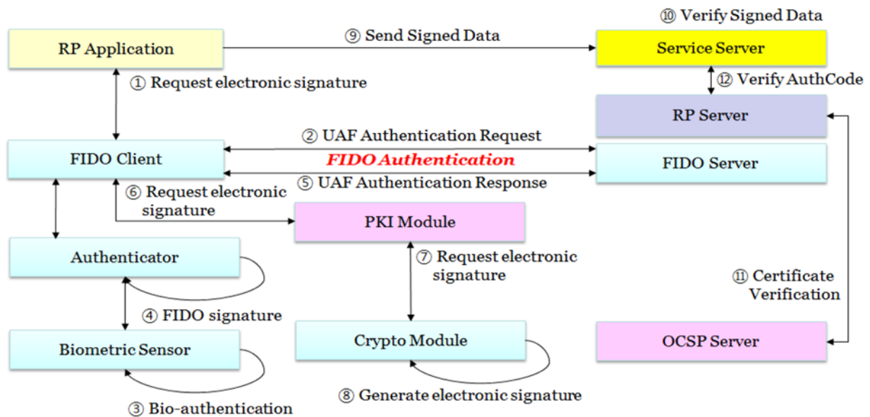
Figure 37 - Authentication Process of K-FIDO Service
