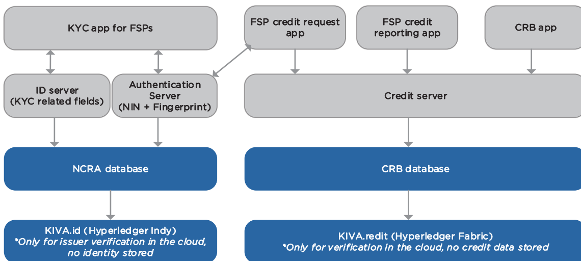
Figure 28 - Digital Credit Reporting Ecosystem Architecture
