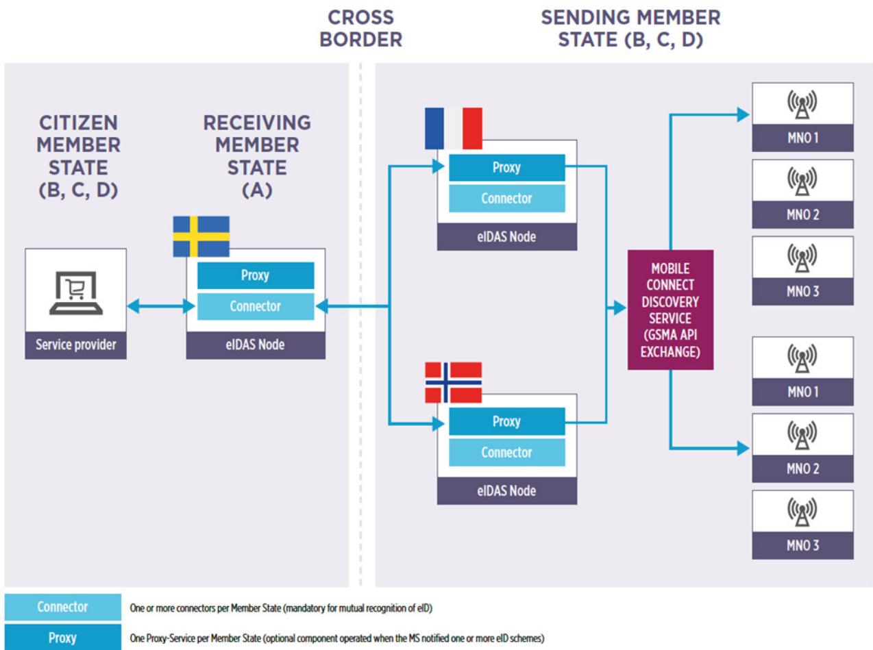
Figure 8 - Mobile Connect and eIDAS reference architecture
