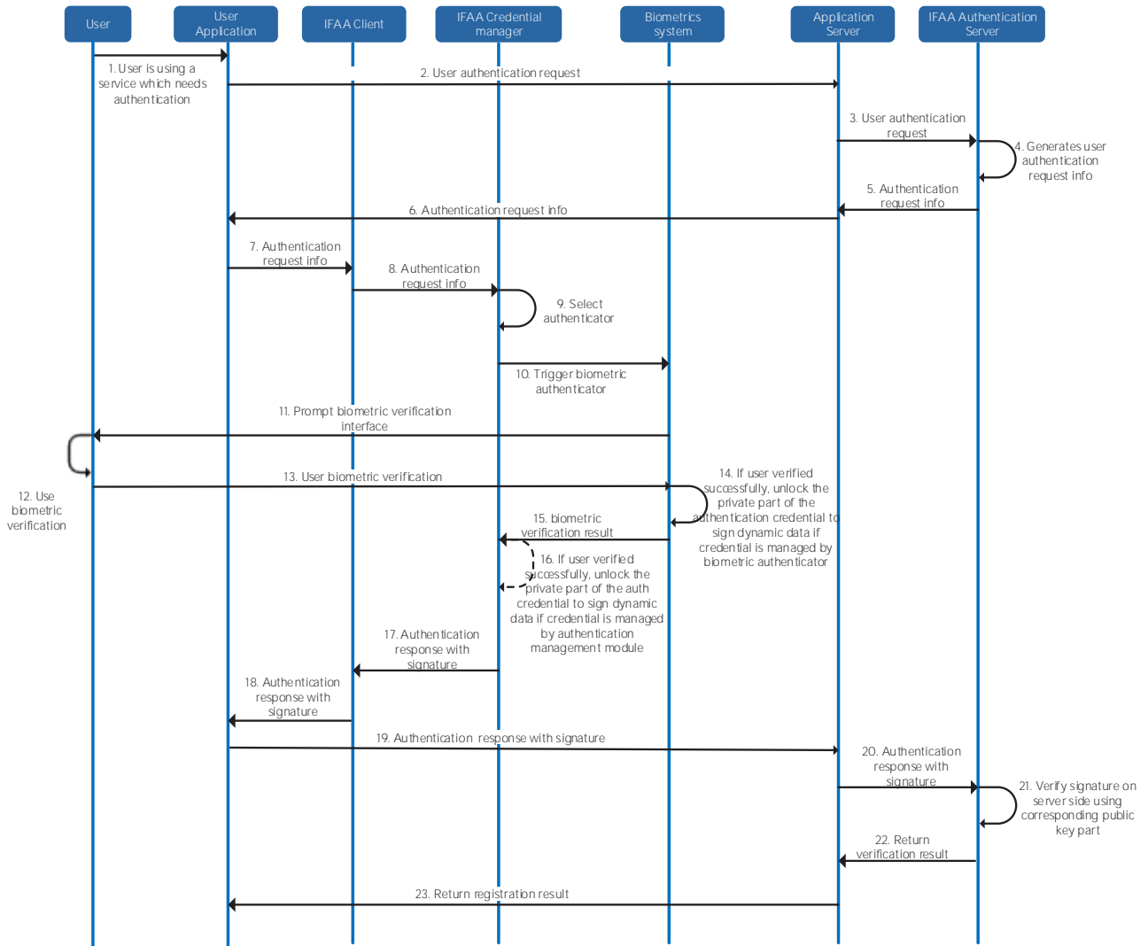
Figure 16 - IFAA biometric authentication - local model - Authentication
