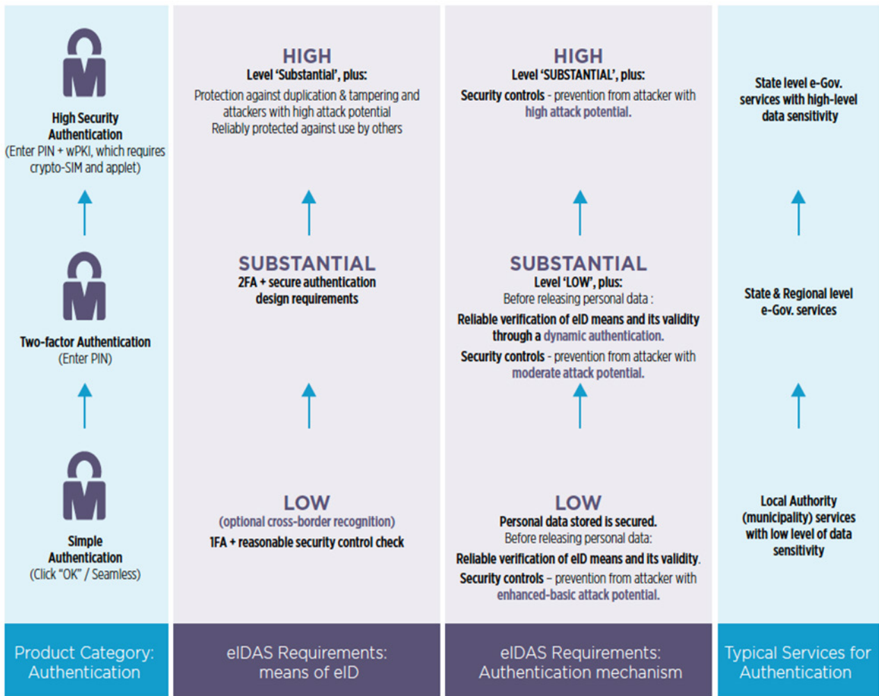
Figure 7 - shows a mapping between Mobile Connect and eIDAS level of assurance.
