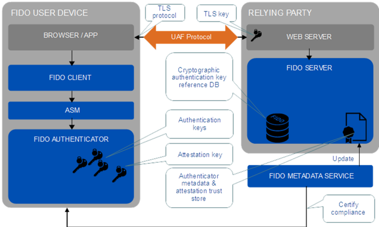
Figure 3 - Universal Authentication Framework Architecture
