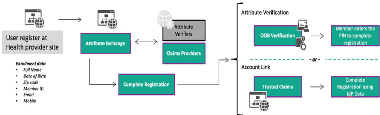
Figure 33 - Healthcare provider user enrolment
