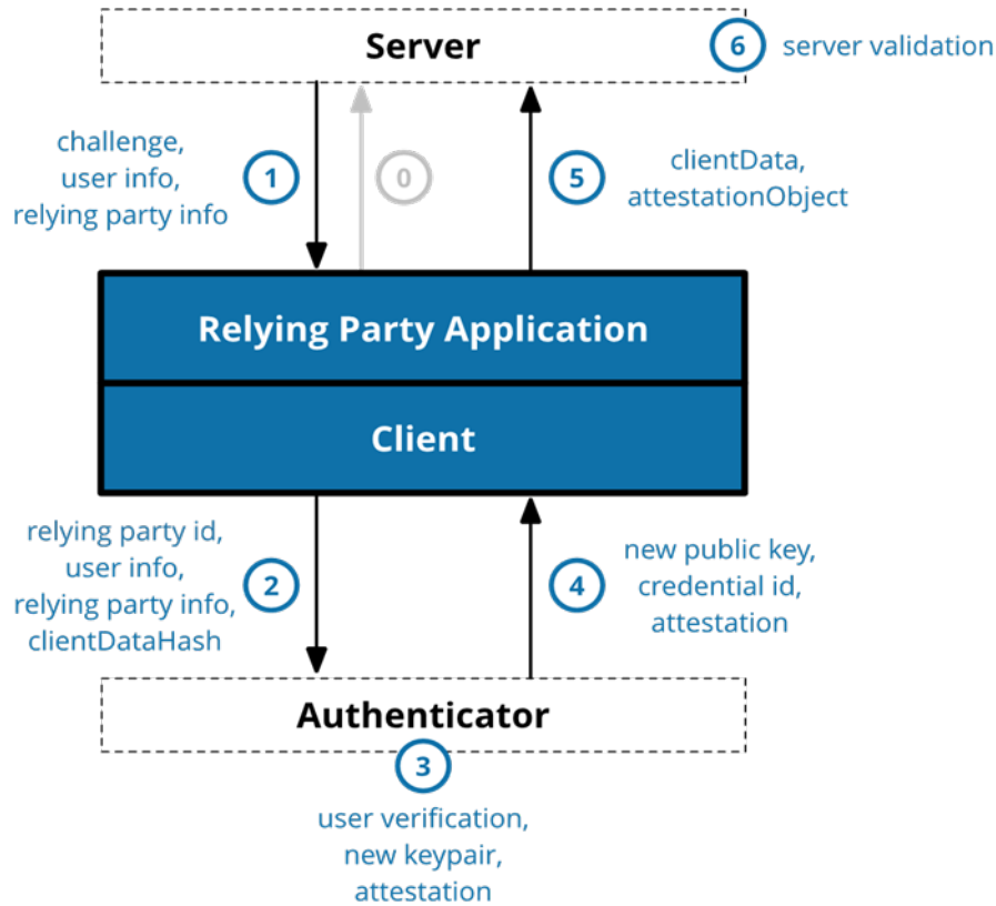
Figure 32 - Registration process of FIDO
