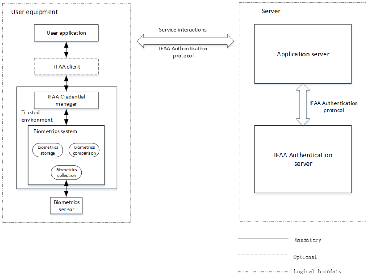
Figure 14 – I FAA biometric authentication – local model
